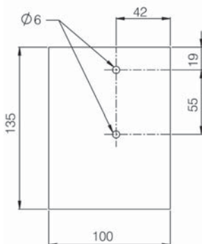
Control Box Installation Template
